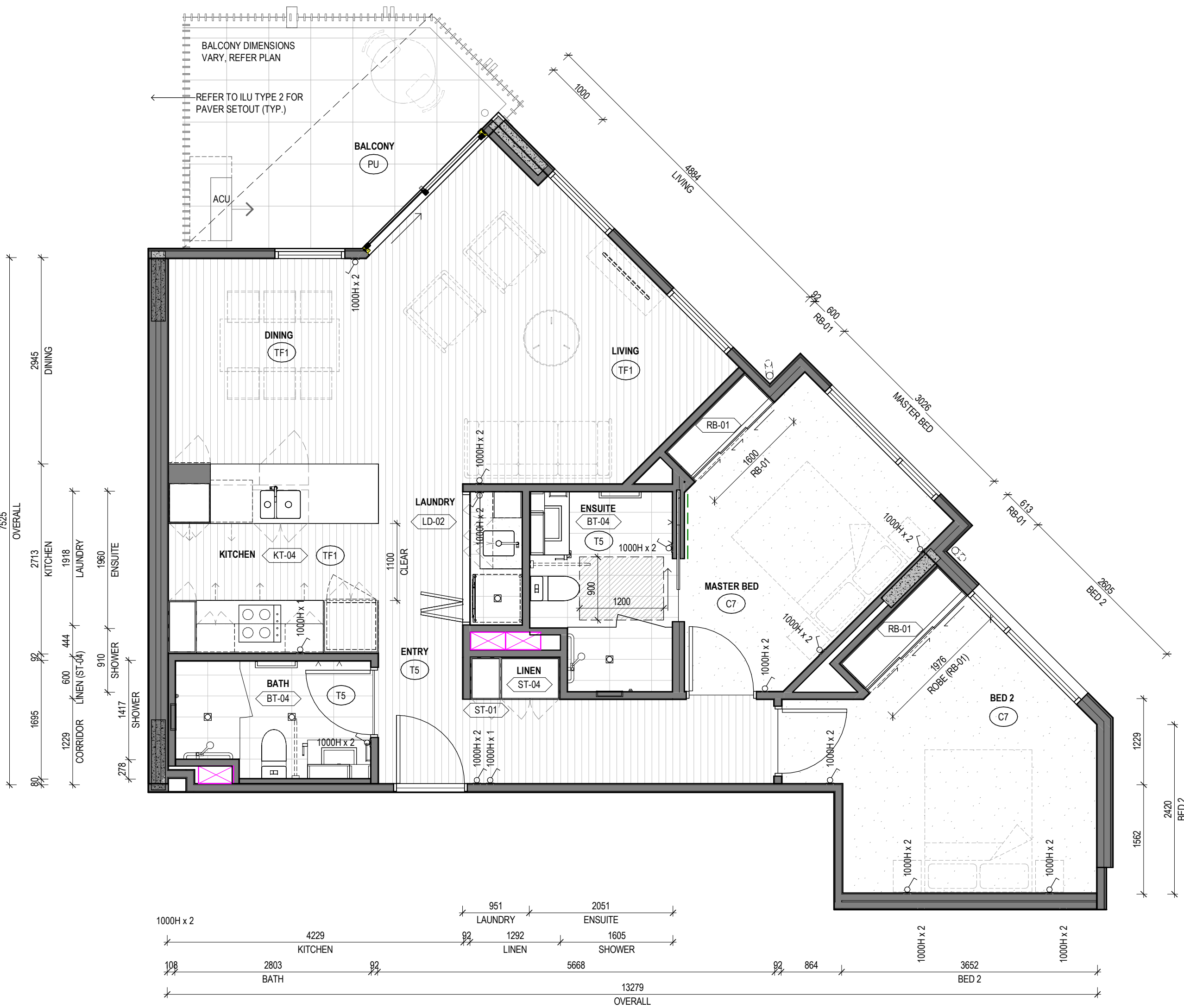
1 ILA Type 5 Scale 1:50
